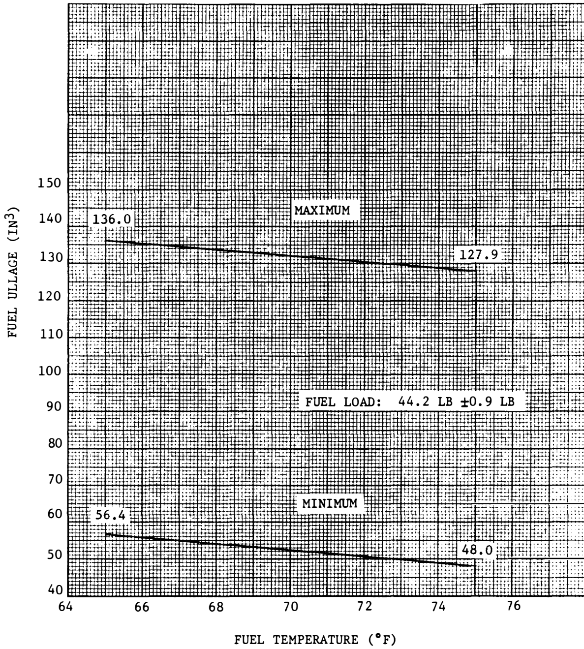
CSM 104 AND SUBSEQUENT CM RCS Figure 4.3-4 FUEL TANK ULLAGE VS TEMPERATURE
