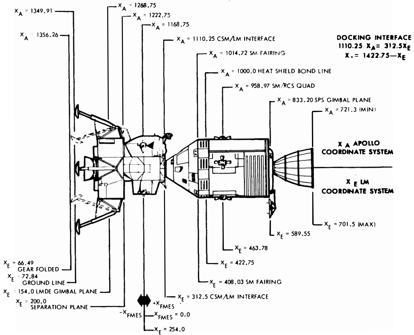
Figure 2-10. CSM/LM Docked Configuration Reference Dimensions
