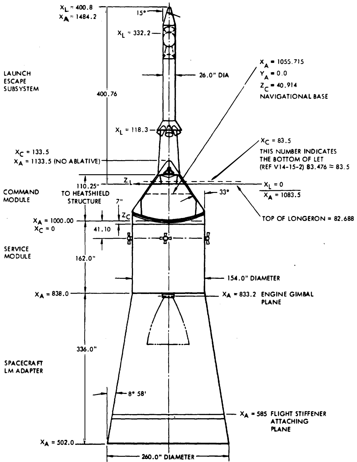
Figure 2-2. Apollo Spacecraft Reference Dimensions
