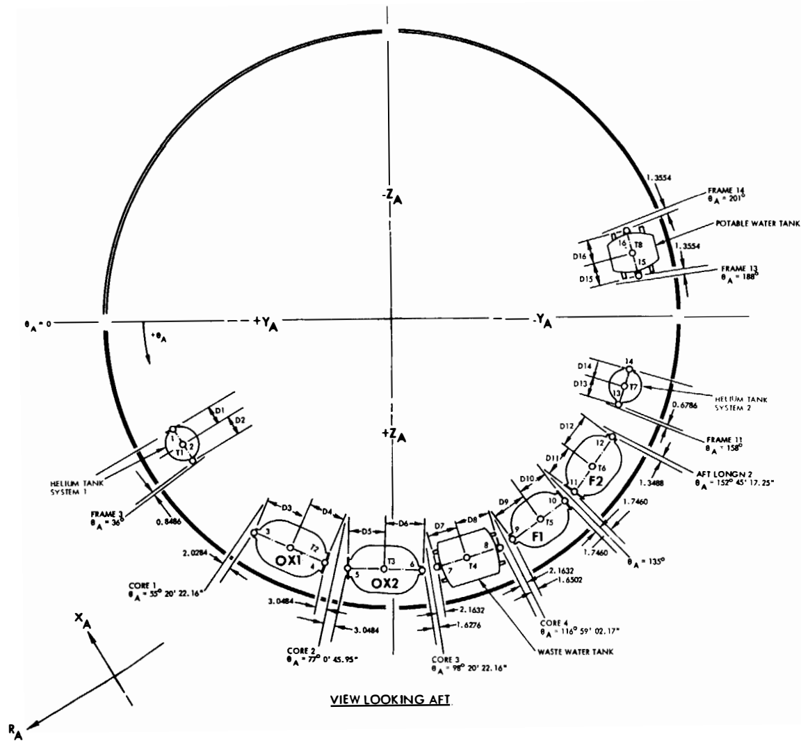
Figure 2-7. CM/RCS TANK LOCATIONS IN APOLLO (X) COORDINATE SYSTEM
