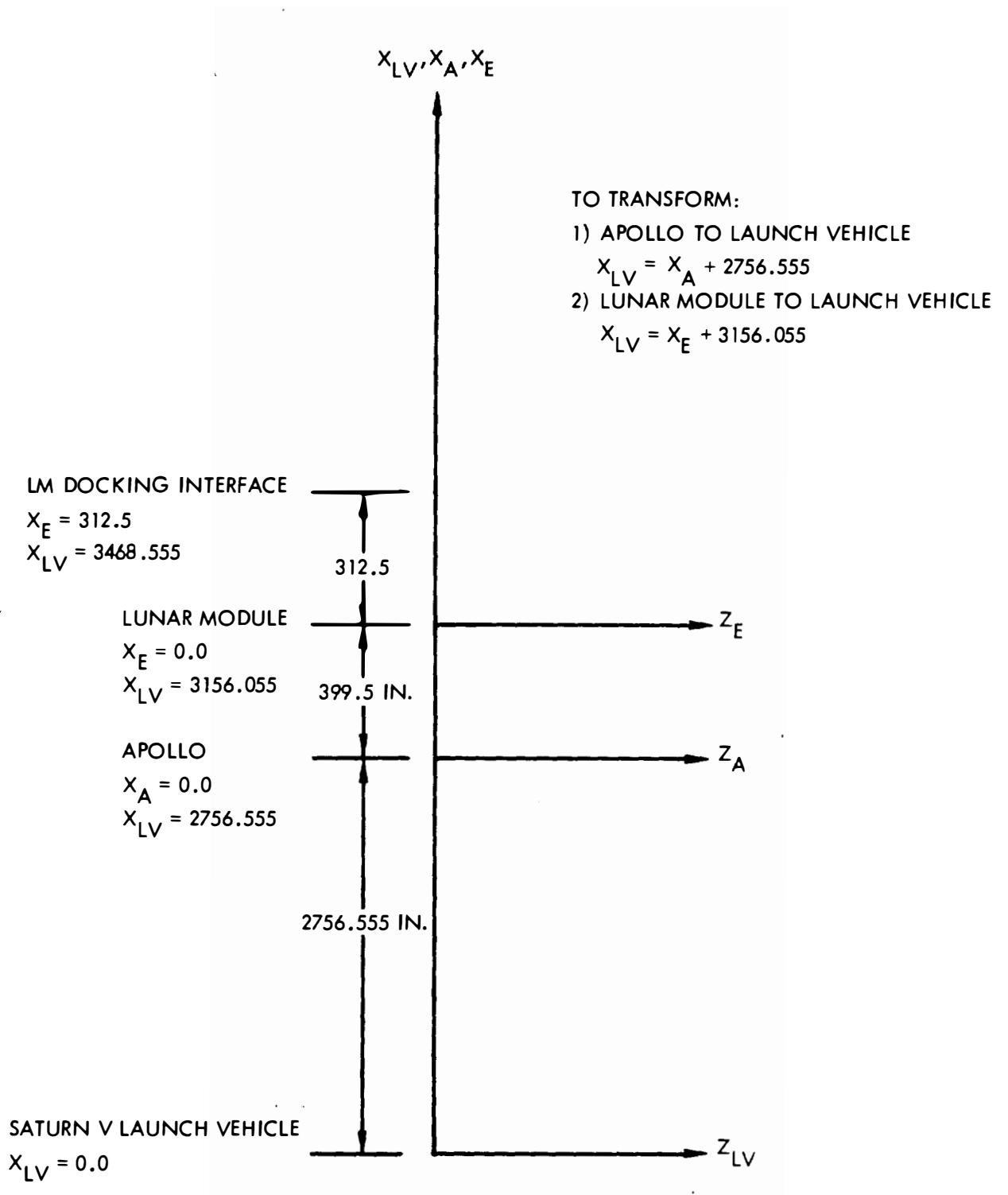
Figure 2-16. Launch Configuration Station Reference
