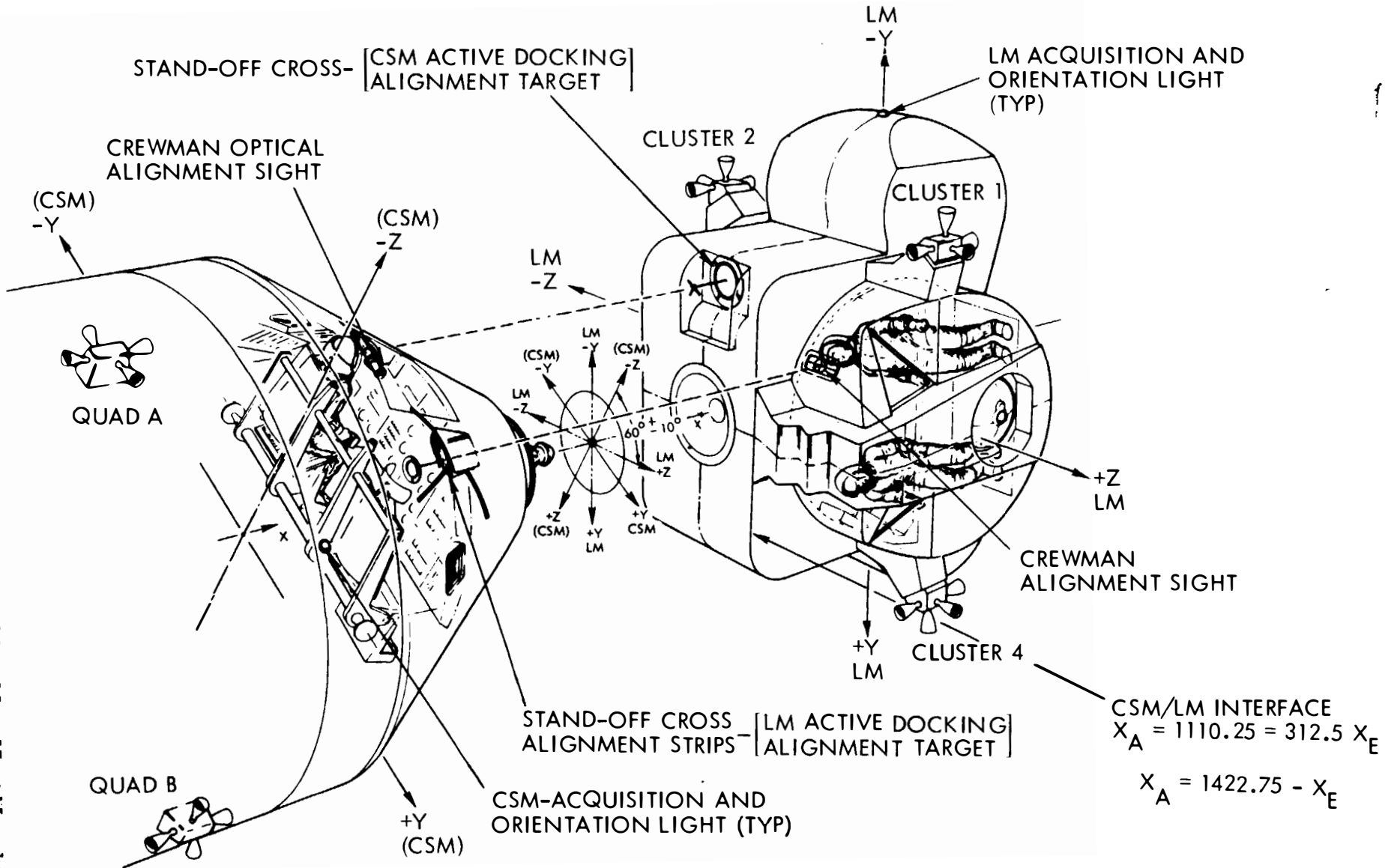
Figure 2-4. LM/CSM DOCKED ORIENTATION
