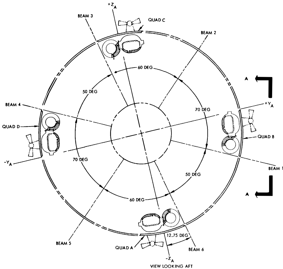
Figure 2-6. SM/RCS TANK LOCATIONS IN CSM ( X_A ) COORDINATE SYSTEM
